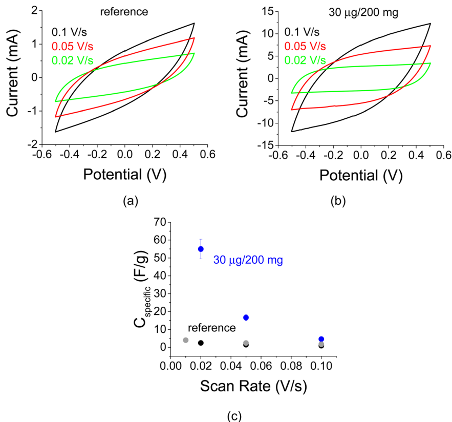
Fig. 11 C–V data as a function of various scan rates for (a) reference sample (no AuNPs) and (b) with 30 µg of AuNPs per 200 mg of AC in a 1 M Na 2 SO 4 electrolyte. (c) The gravitonic specific capacitance as a function of the scan rate. The experiment for the reference sample was repeated twice (the gray and black dots).
