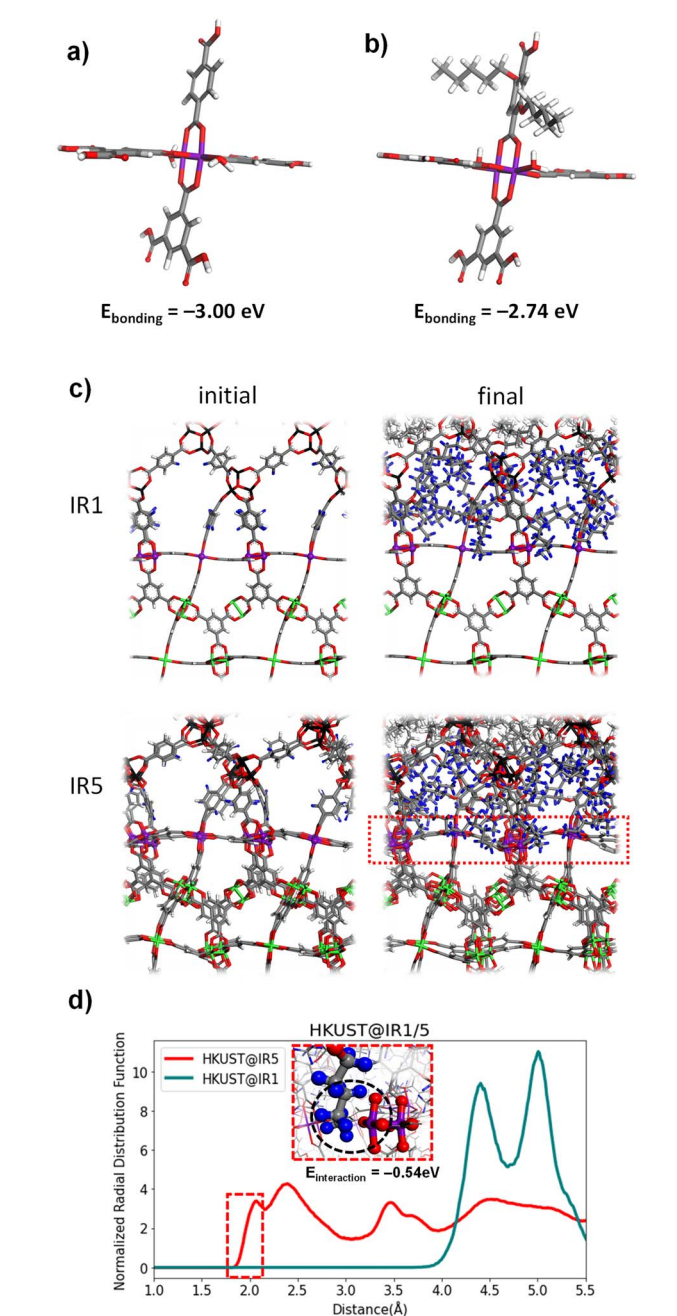
Fig. 2 Bonding energy calculation cluster model for (a) HKUST@IR1 and (b) HKUST@IR5. E_{\text{bonding}} indicates the bonding energy of the external linker to the Cu-paddlewheel interface. (c) The initial and final MD structures of HKUST@IR1 and HKUST@IR5. Green: Cu; black: Zn; grey: C; white: H; red: O; purple: central Cu in the radial distribution function (RDF); blue: distributed H in the RDF. (d) RDF calculation results for HKUST@IR1 and HKUST@IR5. The inset figure indicates the molecular dynamics snapshot of the HKUST@IR5 interface. E_{\text{interaction}} indicates the interaction energy of pentoxy groups and the Cu-paddlewheel.
