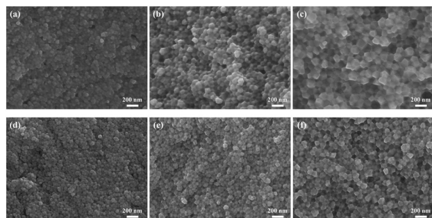
Fig. 6 Cross-sectional SEM images of 5LB1C-3 (a), 5LB1C-2 (b), 5LB1C-1 (c), 5LB-3 (d), 5LB-2 (e), 5LB-1 (f).
