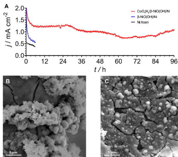
Fig. 5 (A) Long-term chronoamperometric ( E = 1.000 \pm 0.003 V vs. SHE) AOR test of \text{CoO}_x\text{H}_y/\beta\text{-NiOOH}/\text{Ni} (red) in 0.1 \text{ M K}_2\text{HPO}_4 + 0.5 \text{ M NH}_3 . Short-term (6 h) data for \beta\text{-NiOOH}/\text{Ni} (blue) and Ni foam (black) are shown for comparison. Currents are normalised to the geometric surface area of the electrodes ( 1 \text{ cm}^2 ). (B and C) SEM images of the \text{CoO}_x\text{H}_y/\beta\text{-NiOOH}/\text{Ni} electrode (B) as-prepared and (C) after the test shown in panel A.
