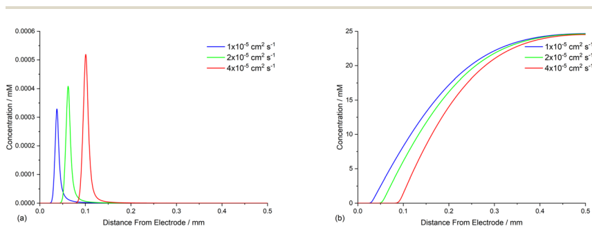
Fig. 5 Influence of mediator ( E^0 = -2.5 \text{ V} vs. SCE) with different diffusion coefficients ( 1 \times 10^{-5} \text{ cm}^2 \text{ s}^{-1} , 2 \times 10^{-5} \text{ cm}^2 \text{ s}^{-1} , and 4 \times 10^{-5} \text{ cm}^2 \text{ s}^{-1} ) on reaction layer detachment. Concentration profiles of: (a) cyclised radical 6 at t = 5 \text{ s} ; (b) ArI 1 at t = 5 \text{ s} .
