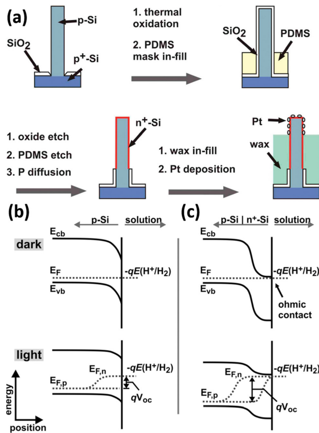
Fig. 26 (a) Schematic diagram of the preparation process of \text{Pt}/\text{n}^+\text{p-Si} wire arrays. Band bending of (b) \text{p-Si} and (c) \text{n}^+\text{p-Si} photocathodes in contact with electrolyte. Reproduced with permission from ref. 68, Copyright © 2011, American Chemical Society.
