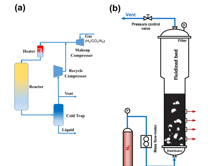
Fig. 14 (a) Schematic flow diagram of the pilot-scale fixed-bed reactor, 49 (b) schematic diagram of the cold-flow apparatus. 110 Reproduced from ref. 49 and 110 with the permission from Springer Nature and Wiley, copyright 2017 and 2022.
