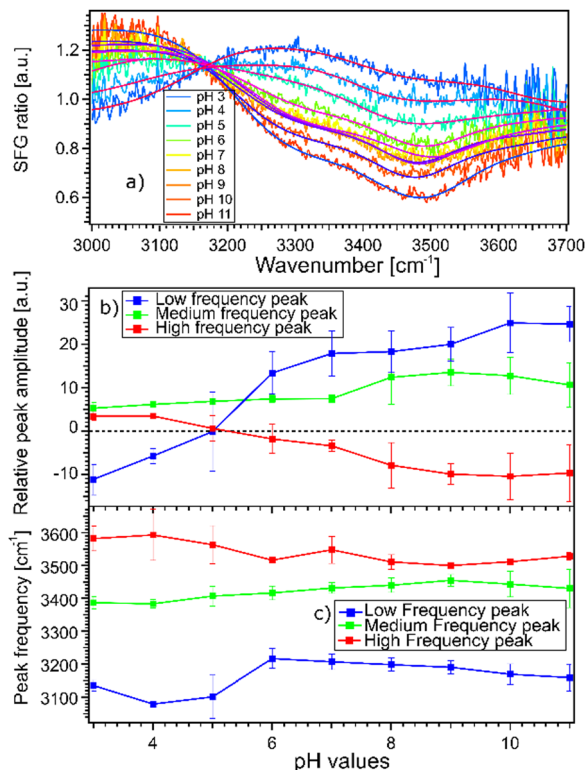
Fig. 3 (a) SFG spectra for the STO–water pH 3 to pH 11 interface, normalized by the STO–D 2 O interface, at position 2 on the layer together with the fitting curves obtained by the Lorentzian lineshape model. Here position 2 is chosen as a representative position. (b) Amplitude of each peak obtained from fitting pH dependent SFG-spectra acquired at 3 different positions. (c) Central frequency of each of the three peaks as a function of pH. The error bars indicate the standard deviation of the three datasets.
