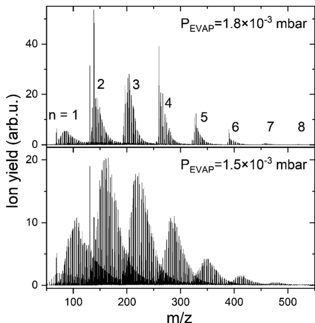
Fig. 1 Mass spectra showing H_mCu_n^+ ions extracted from multiply charged HNDs doped with ^{63}Cu via multiple collisions with H_2 gas at a pressure of 1.8 \times 10^{-3} (top) and 1.5 \times 10^{-3} (bottom) mbar. The number n of Cu atoms in the ions is indicated by the numbers on top of the pronounced peak series.
