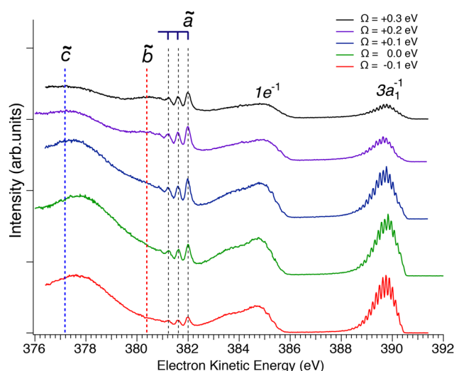
Fig. 2 Resonant Auger spectra taken at several photon energy values across the N 1s -1 4a 1 resonance. The different spectra are measured at different values of detuning \Omega , which is the difference between the photon energy and the energy corresponding to the highest core-excitation cross section for the N 1s -1 4a 1 resonance (400.66 eV). The theoretically expected energy positions for the different Auger transitions in NH 2 + fragment are also indicated based on the energy differences between the states \tilde{a}^1A_1 as well as \tilde{b}^1B_1 and \tilde{c}^1A_1 of the NH 2 + ion with the H–N–H bond angle of 110°, which corresponds to the geometry of the core-excited fragment. 32 All spectra are normalized to photon flux and acquisition time.
