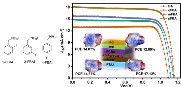
Fig. 11 J - V curve confirming the best performance for the (4-FBA) _2 -MA _4 Pb _4 I _6 PV device in an inverted configuration. 73 ESPs are shown in the inset (unit a.u.). Reproduced with permission from ref. 73. Copyright 2022, American Chemical Society.
