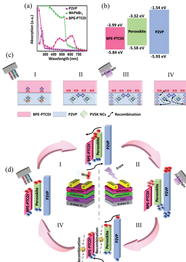
Fig. 11 (a) Absorption spectra of n-type BPE-PTCDI, perovskite MAPbBr 3 , and polymer matrix P2VP. (b) The respective energy bands. (c) Charge migration upon photo-writing (charging) and photo-recovery (neutralizing) processes on the fully optical driven photonic memory transistor. (d) Schematic energy band diagrams in association with the photo-writing and photo-recovery processes. Reprinted with permission from ref. 36. Copyright 2021 American Chemical Society. 36
