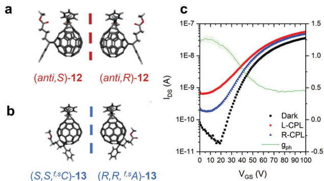
Fig. 5 (a) and (b) Molecular structures of enantiopure bis-PC 61 BM ( anti,S/R )- 12 and ( S,S/R,R,f5C/A )- 13 . (c) Variation of transfer curves of ( anti,R )- 12 upon exposure to LH and RH CPL (95 mW cm -2 ), compared to curves in the dark. V_D = 20 V. Dissymmetry factors for the photocurrent generation ( g_{ph} ) and its associated error are given by the green curve and shaded area, respectively. Reproduced with permission from ref. 42. Copyright 2021, Wiley-VCH.
