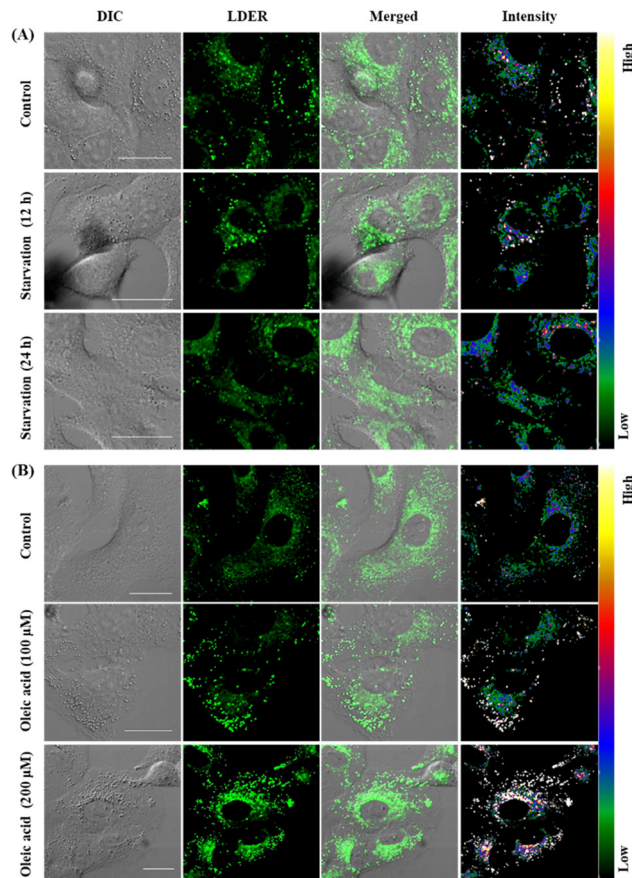
Fig. 6 (A) Fluorescence images of SiHa cells incubated in nutrient-free medium for different times, followed by staining with LDER (5 \mu\text{M} ); (B) fluorescence images of SiHa cells stained with LDER (5 \mu\text{M} ) after the cells were pretreated with different concentrations of oleic acid for 4 h. The rainbow of color represents the fluorescence intensity. Scale bar = 20 \mu\text{m} .
