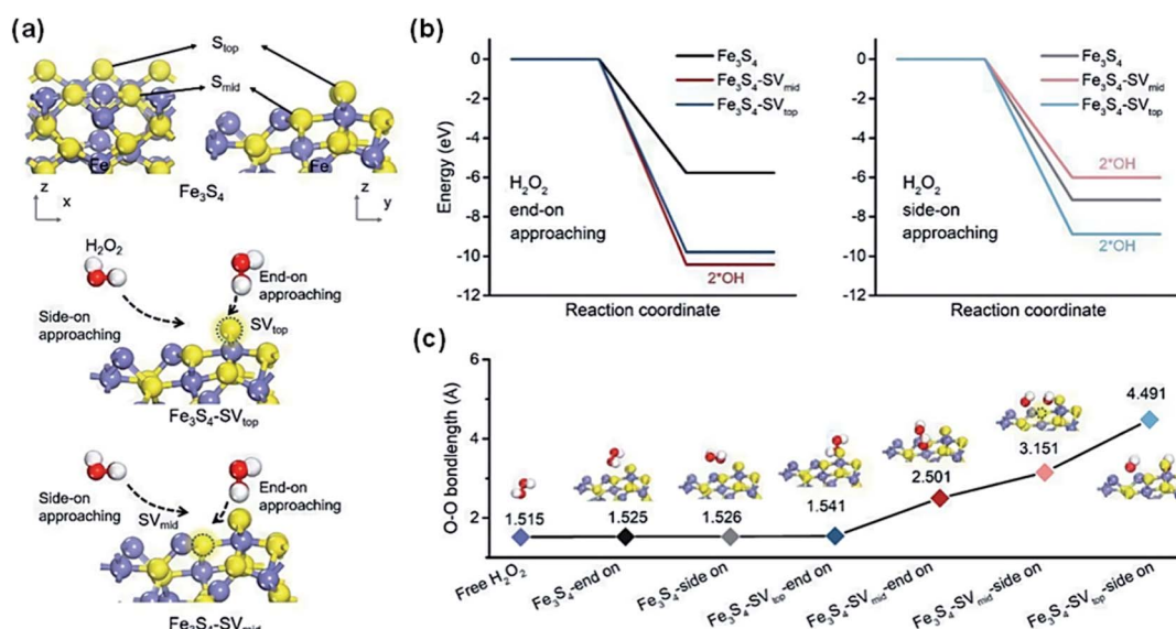
Fig. 2 (a) Models of Fe_3S_4 and SVs-rich Fe_3S_4 with exposure of the (011) surface. (b) Energy diagrams of H_2O_2 adsorption on SVs-rich Fe_3S_4 via end-on and side-on attachment models. (c) The O–O bond length of adsorbed H_2O_2 in different adsorption configurations. Adapted with permission from ref. 110 Copyright (2021) Elsevier.
