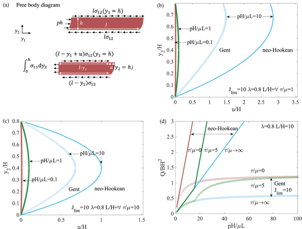
Fig. 9 (a) Free body diagram of the seal with friction at the top. (b and c) Displacement u of seal materials at height of y_2 . \tau/\mu is the dimensionless friction on the upper boundary. (d) p - Q curves for both strain-stiffening (Gent) and neo-Hookean seals when friction at the top surface of the seal is considered, assuming no leak happens.
