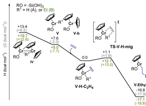
Fig. 5 Calculated reaction enthalpies ( H kcal mol ^{-1} ) and free energies ( G kcal mol ^{-1} ) for potential ethylene activation pathways involving monomeric Cr(III) hydrides such as V (in black), or monomeric Cr(III) alkyl species such as V-ethyl (in green). Ethylene activation and chain propagation are both associated with reasonable energy costs.
