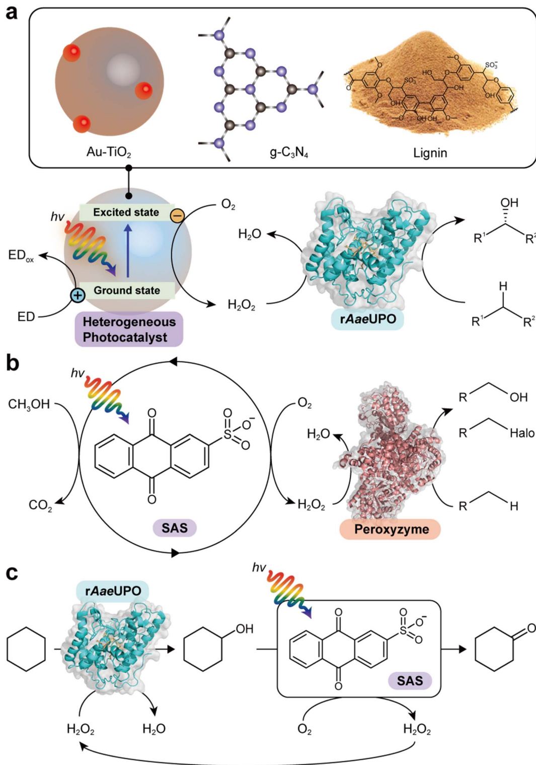
Fig. 6 Photocatalytic formation of H 2 O 2 and selective oxidation reactions catalyzed by rAaeUPO and peroxymzyme. Representative photocatalysts include Au-TiO 2 , 90 g-C 3 N 4 , 95 lignin 99 (a), and anthraquinone (SAS) 97,106 (b). (c) Photocatalytic oxidation of cyclohexane to cyclohexanone. The SAS-catalyzed aerobic overoxidation of cyclohexanol to cyclohexanone produces H 2 O 2 as a byproduct, which itself is used to support the rAaeUPO-catalyzed hydroxylation of cyclohexane. 97
