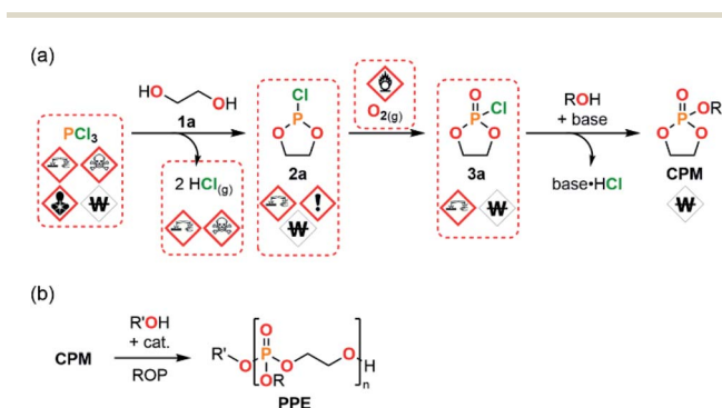
Fig. 1 (a) 3-step synthetic pathway commonly used for the preparation of CPMs involving hazardous and/or sensitive reactants, intermediates and by-products. (b) Ring-opening polymerization strategy used for the production of PPEs starting from CPMs.
