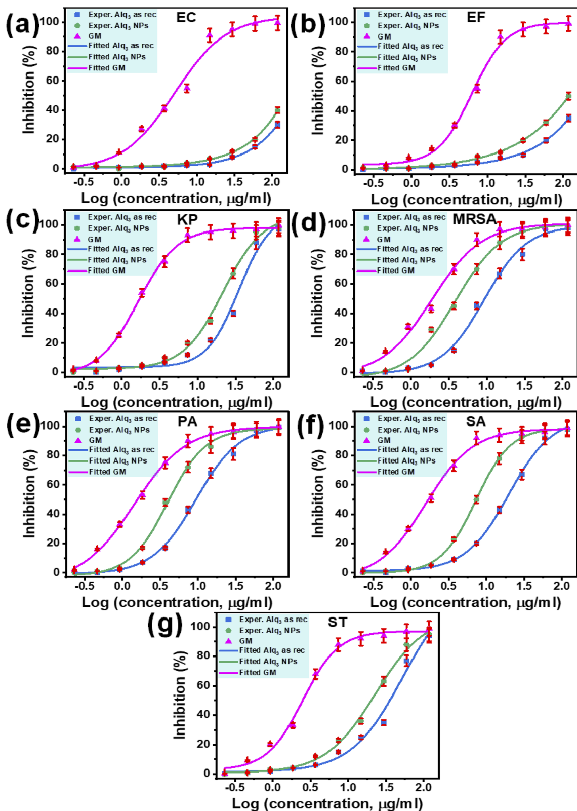
Fig. 6 Bacterial growth inhibition experimentally from the Alq 3 as rec sample, Alq 3 NP sample, and St. aureus antibiotic GM versus common logarithms of the concentrations of 120, 60, 30, 15, 7.5, 3.75, 1.88, 0.94, 0.47, and 0.23 \mu\text{g ml}^{-1} against (a) EC, (b) EF, (c) KP, (d) MRSA, (e) PA, (f) SA, and (g) ST. The lines are the fitted dose-response curves.
