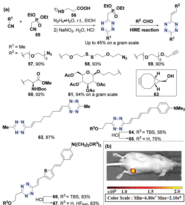
Fig. 8 Synthesis of alkyl-substituted tetrazines via the tetrazine-HWE reaction. (a) Synthesis method. (b) In vivo imaging of probe 67 . Adapted from ref. 79 with permission from John Wiley and Sons.
