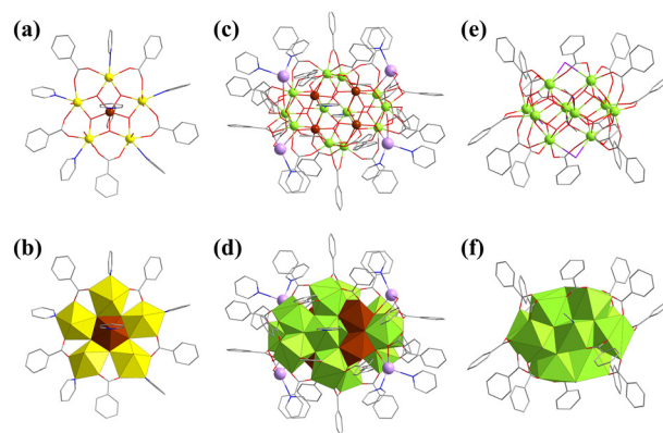
Fig. 21 Views of (a and b) [U(UO_2)_5(\mu_3-O)_5(PhCOO)_5(Py)_7] , (c and d) \{[K(Py)_2]_2[K(Py)]_2[U_{16}O_{24}(PhCOO)_{24}(Py)_2]\} , (e and f) [U_{10}O_8(OH)_6(PhCO_2)_{14}I_4(H_2O)_2(MeCN)_2] . Color codes: U IV , green; U V , brown; U VI , yellow; I, violet. Other color codes are the same as in Fig. 1.
