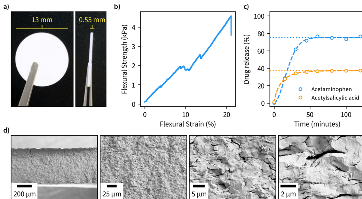
Fig. 4 Application of hexagonal \beta -1,3-glucan microparticles synthesized at 50 °C as drug encapsulation tablets. (a) Tablets compressed from freeze-dried \beta -1,3-D-glucan ( 80 mg dry weight). (b) Flexural stress and strain properties of the compressed tablets. (c) Release profiles of tablets containing 5 mg acetaminophen or acetylsalicylic measured during incubation of tablets in phosphate buffer (pH 7) at 37 °C, with a dashed line indicating a fit for the drug release obtained using Weibull function and a dotted line indicating the cumulative amount of drug released at infinite time corresponding to the fit. (d) SEM images at different magnifications of the cross-sectional view of fractured specimens after bending test.
