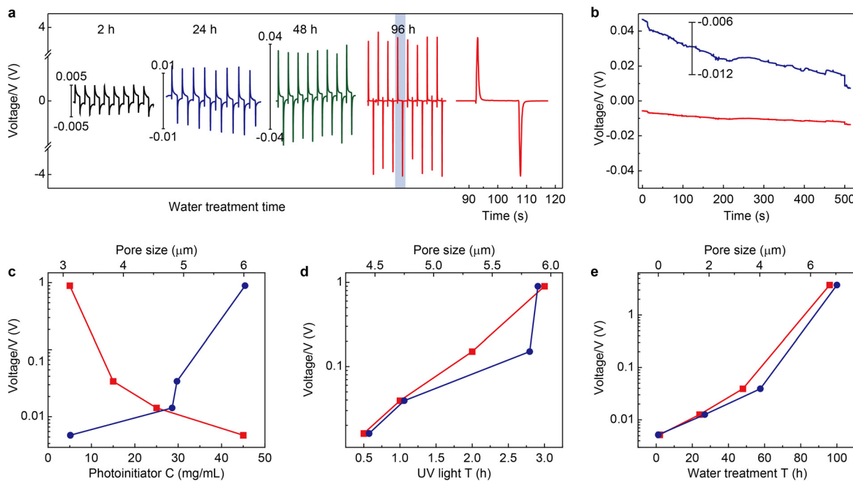
Fig. 4 Output characteristics of the magnetic energy harvesting device. (a) Time-dependent output voltages of the devices fabricated by using magnetic polyionic liquid micropores synthesized with different water treatment times. The voltage scales for 2 h (black curve), 24 h (blue curve), and 48 h (green curve) devices are given on the left side of the curves. The 96 h device (red curve) uses the left y-axis. The time interval of each cycle is 30 s. The far-right curve is the magnified one cycle in the 96 h device. Note: the distinct waveform and significant enhancement of output voltage between 96 h and others are probably due to the changes in the pore structure, including the pore size and through-hole channel structure. (b) A similar experiment is performed by using non-magnetic polyionic liquid micropores ( [\text{HS-C}_{10}\text{mim}]\text{NO}_3 ). The blue curve is the magnified view of the time-dependent output curve. The output voltage amplitude of devices as a function of (c) photoinitiator concentration (bottom x-axis, red markers) and the corresponding pore size (top x-axis, blue markers), (d) UV irradiation time (bottom x-axis, red markers) and the corresponding pore size (top x-axis, blue markers), and (e) water treatment time (bottom x-axis, red markers) and the corresponding pore size (top x-axis, blue markers).
