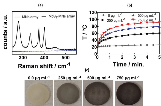
Fig. 3 Characterization of the MoS 2 -MN array formed from a GelMA : PEDGMA (20 : 10) cocktail using different amounts of MoS 2 : (a) Raman spectrum of the GelMA : PEDGMA hydrogel loaded with 500 \mu\text{g mL}^{-1} of MoS 2 . (b) Photothermal heating properties of the MoS 2 -MN array under irradiation with a laser at 980 nm ( 1.0 \text{ W cm}^{-2} ) as a function of MoS 2 amount in the hydrogel cocktail. (c) Photographic images of the MNs with increasing amounts of incorporated MoS 2 .
