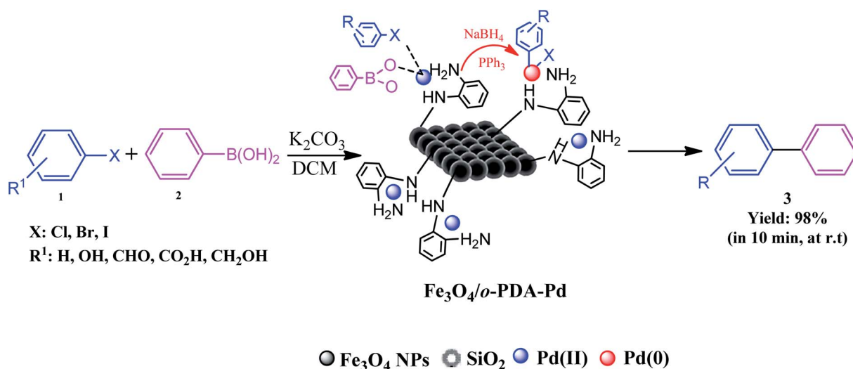
Fig. 27 Schematic of Suzuki-Miyaura cross-coupling reaction conducted using magnetic Fe 3 O 4 / o -PDA-Pd nanocatalyst at room temperature (r.t). This figure was adapted with permission from Journal of Physics and Chemistry of Solids , 2020, 136 , 109200. 17
