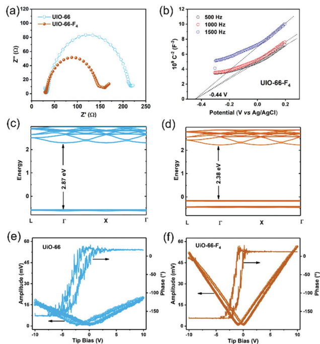
Fig. 3 (a) Electrochemical impedance spectra of UiO-66 and UiO-66-F 4 . (b) Mott-Schottky plots of UiO-66-F 4 at different frequencies. DFT calculation of the band structures of (c) UiO-66 and (d) UiO-66-F 4 . PFM phase and amplitude hysteresis loops of (e) UiO-66 and (f) UiO-66-F 4 .
