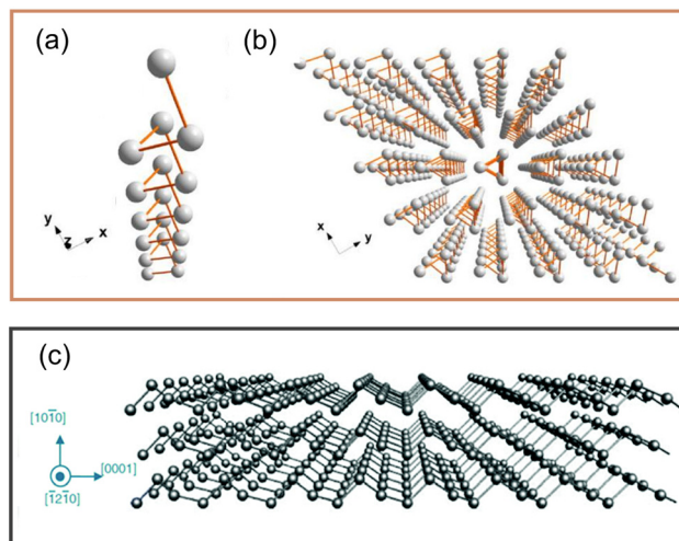
Fig. 2 (a) Structure of single-molecule Te chain. 47 (b) Crystal structure of Te. 47 Copyright 2018, American Chemical Society. (c) Structure of tellurene. 17 Copyright 2019, Royal Society of Chemistry.
