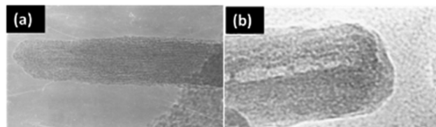
Fig. 14 \text{MoSe}_2 nanotubes obtained via decomposition of (a) \text{MoSe}_2 and (b) (\text{NH}_4)_2\text{MoSe}_4 . Reprinted with permission from ref. 94 [M. Nath and C. N. Rao, Chem. Commun. , 2001, 2236–2237]. Copyright The Royal Society of Chemistry.
