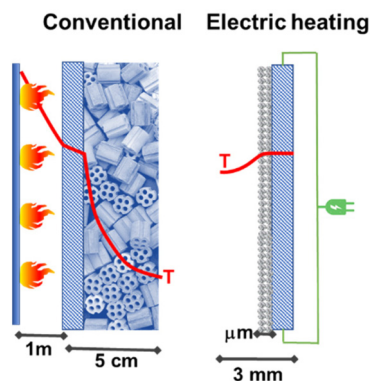
Fig. 4 Conventional fired reactor versus electric resistance-heated reactor with an indication of the radial temperature profiles. Adapted from ref. 45 with permission. Copyright © 2019, The American Association for the Advancement of Science.
