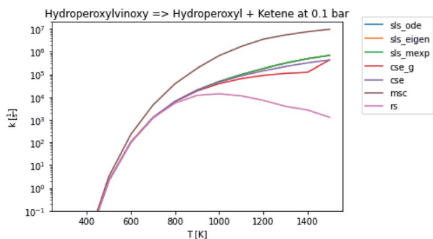
Fig. 7 Rate coefficient for hydroperoxyvinoyx to hydroperoxyl and ketene at 0.1 bar.
