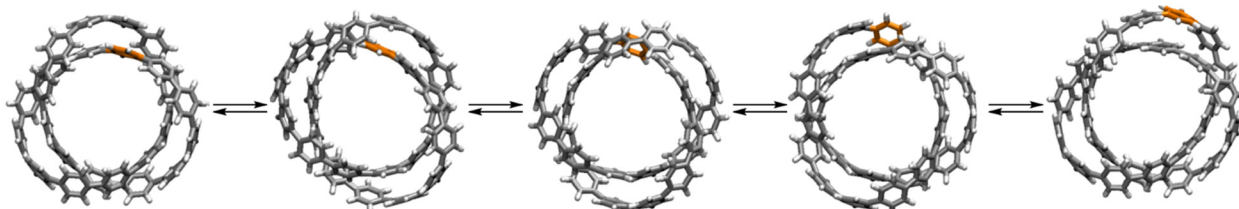
Fig. 30 Entanglement dynamics of all-benzene trefoil knot \mathbf{62} as illustrated with snapshots from DFTB-MD simulations. 91
