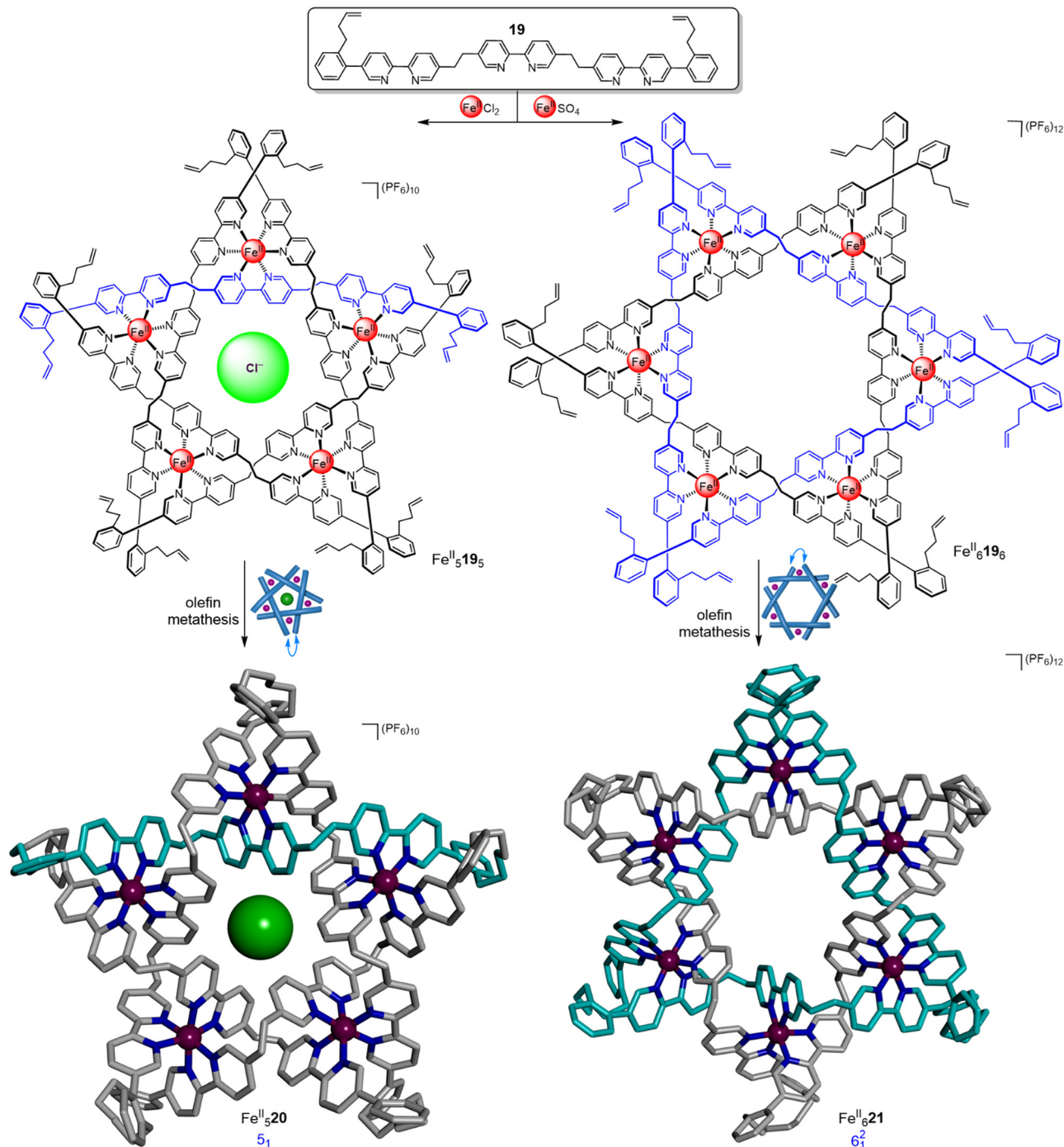
Fig. 7 Generation of hexameric and pentameric circular helicates and their subsequent closure by olefin metathesis to form a pentafoil knot \text{Fe}^{\text{II}}_5\mathbf{20}_{5_1} and a Star of David triply interlocked [2]catenane \text{Fe}^{\text{II}}_6\mathbf{21}_{6_1^2} . 56
