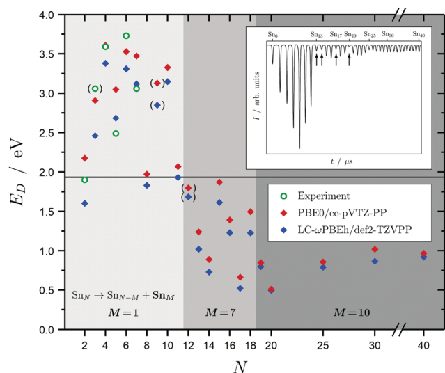
Fig. 2 Dissociation energies E_{\text{D}} in eV for the energetically most favorable fragmentation channels of the Sn N clusters with N = 2 –20, 25, 30, 40 averaged over all isomers in the given energy range. Experimental values for the incremental dissociation energies are estimated based on atomization enthalpies obtained from Knudsen cell mass spectrometry. 14 The horizontal line at 1.9 eV gives the smallest accessible single-photon energy available in our photodissociation experiment. Over the size range studied, three regions can be distinguished: dissociation under the loss of an atom (light gray), a Sn 7 (gray) and a Sn 10 fragment (dark gray). Calculated dissociation energies in parentheses point to a differing fragmentation mechanism, i.e. , loss of a Sn 2 fragment for the Sn 9 parent cluster and loss of Sn 6 fragments for the Sn 12 parent cluster. The Sn 3 experimental dissociation energy in parenthesis has been evaluated assuming a linear geometry 12 (in its lowest 1 A 1 and 3 B 2 state Sn 3 is an isoscele triangle 21 ) and has thus to be considered with care. The inset shows a typical time-of-flight mass spectrum after F 2 excimer laser photoionization (7.89 eV) of the Sn N clusters given as arbitrary intensity I in dependence of the flight time t ; the naturally low-abundant clusters Sn 13 , Sn 14 , Sn 17 and Sn 20 are highlighted by arrows.
