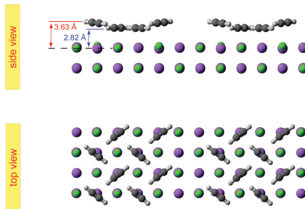
Fig. 5 Best-fit geometry obtained from LEED analysis of structure model A in top view and side view.
