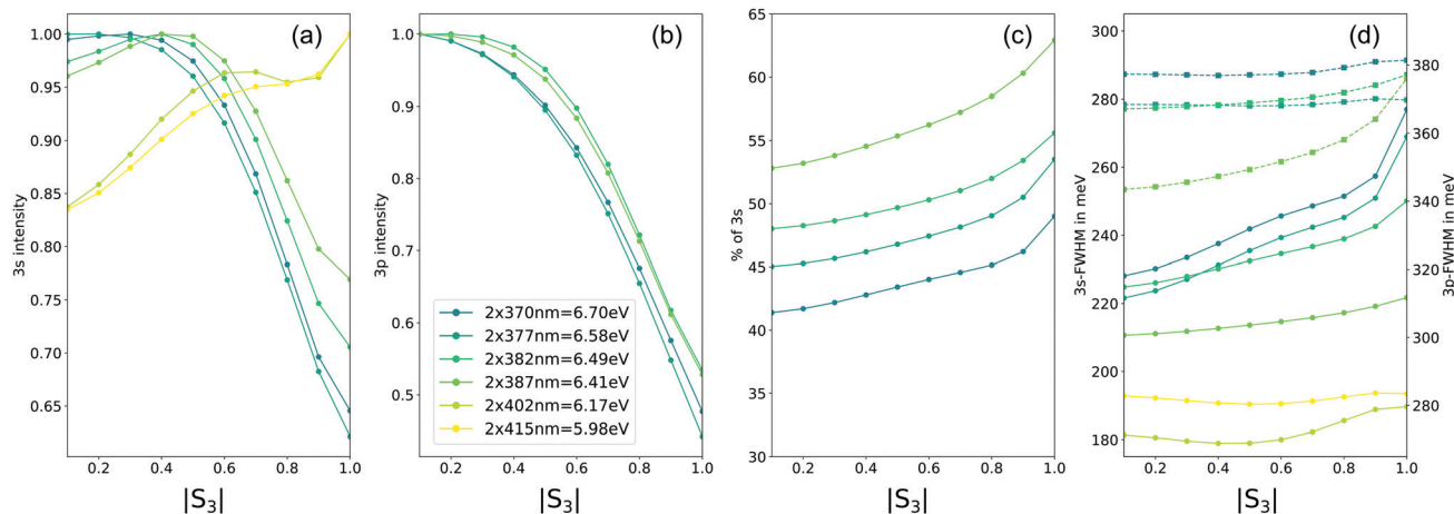
Fig. 10 The PES(b_0) has been fitted by a sum of Gaussians for each |S_3| and wavelength to monitor at which |S_3| the electron yield of (a) the 3s channel maximizes, (b) the 3p channel, or (c) the percentage of the 3s/(3s + 3p) in the PES, as well as (d) Bandwidths of 3s-mediated (full lines, left scale) and 3p-mediated (dashed lines, right scale) of these photoelectron bands.
