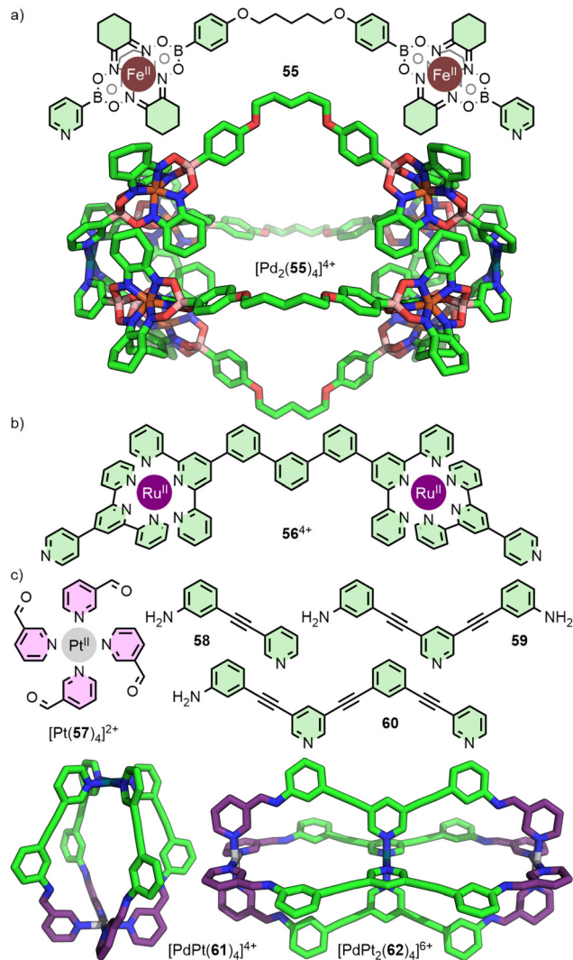
Fig. 11 Kinetically stable metallo-ligands such as (a) Fe(II)-clathrochelate 55 (SCXRD structure), and (b) bis-Ru(II) 56 4+ , each assemble with Pd(II) to give symmetrical Pd_2L_4 systems. (c) In contrast, the use of a subcomponent self-assembly strategy has allowed M_2L_4 and M_3L_4 cages (SCXRD structures) to be accessed in which Pd(II) and Pt(II) ions occupy distinct structural sites within these architectures, despite both residing in tetrapyrrolyl coordination environments.
