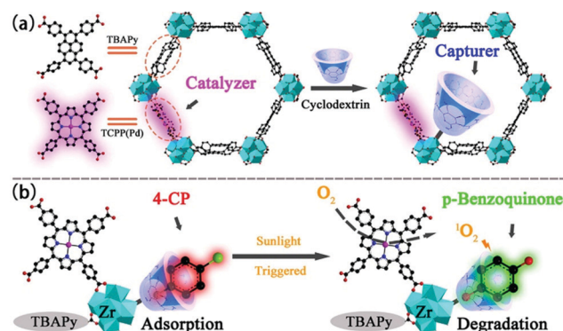
Fig. 15 (a) The construction of CMCD@NU-1000-TCCP(Pd) and (b) schematic illustration of the adsorption and degradation processes toward 4-CP. Reproduced from ref. 170 with permission from American Chemical Society, copyright 2021.
