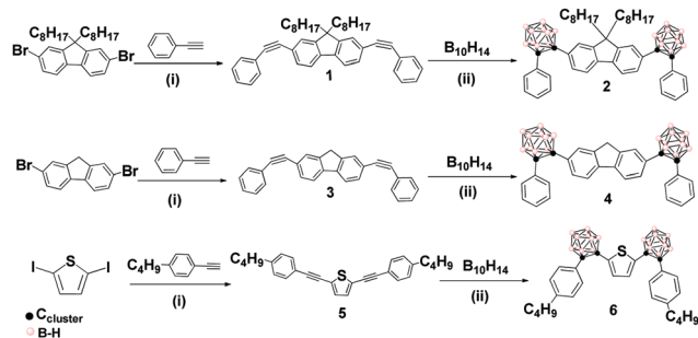
Scheme 1 Synthesis of fluorene- and thiophene-based \pi -conjugated systems linked to o -carborane clusters: (i) Pd(PPh 3 ) 2 Cl 2 , Cul, TEA and toluene (1:9 v/v); (ii) 5 eq. Et 2 S, toluene, 72 h, and 110 °C.
