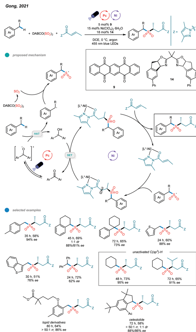
Scheme 21 Photoredox and nickel dual-catalyzed three-component sulfonylations of C–H bonds of alkylbenzenes.
