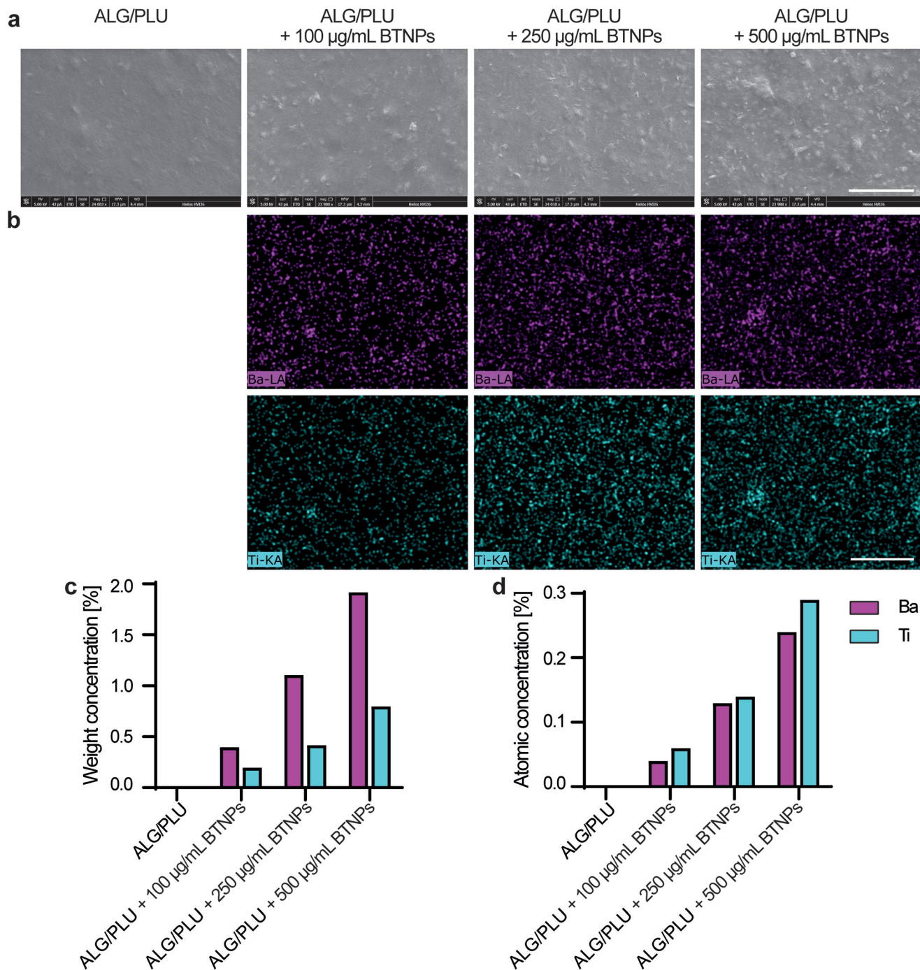
Fig. 4 (a) Representative SEM images of bare and doped printed structures from a top view. Scale bar: 5 µm. (b) Representative EDX analysis images, showing the presence of Ba (in pink) and Ti (in light blue). Scale bar: 5 µm. (c) Quantitative EDX detection of the two elements (Ba and Ti) in terms of weight concentration % and (d) atomic concentration %, on the representative images. ALG/PLU: alginate/Pluronic-based bioink. BTNPs: barium titanate nanoparticles. Ba: barium. Ti: titanate.
