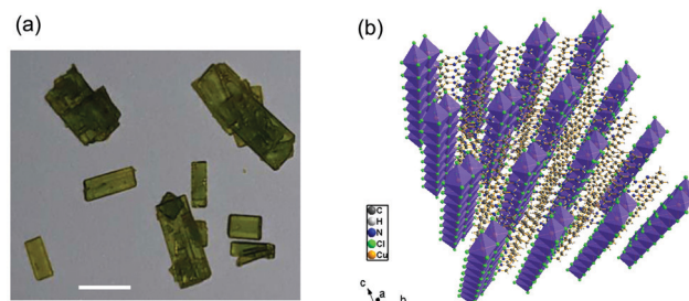
Fig. 1 (a) Microscopy image of the microcrystals (scale bar, 25 μm) and (b) perspective view of the structure of (C 5 H 8 N 3 )[CuCl 3 ].
