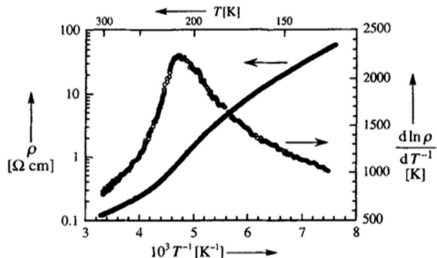
Fig. 4 Electrical resistivity \rho of (\text{DT-TTF})_2[\text{Au}(\text{mnt})_2] ( 1 ) as a function of the reciprocal temperature (left) and its first derivative, d \ln \rho / dT^{-1} (right). Reproduced with permission from ref. 27. Copyright 1997 Wiley-VCH.
