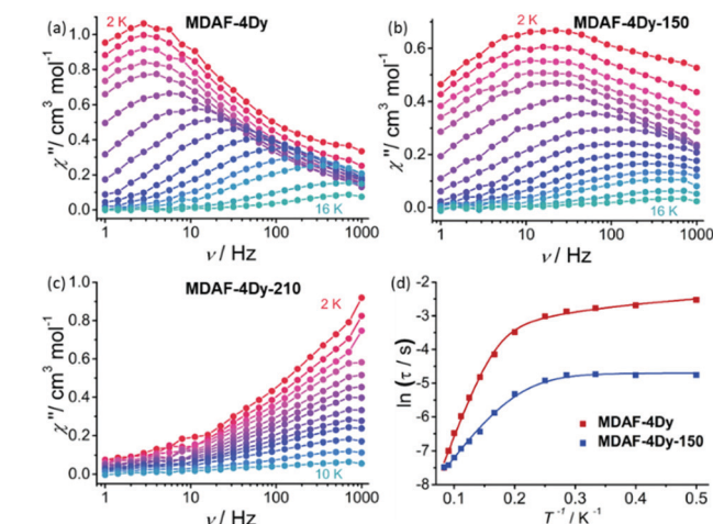
Fig. 6 Frequency dependence of the \chi'' signals measured under zero dc field for (a) MDAF-4Dy , (b) MDAF-4Dy-150 and (c) MDAF-4Dy-210 at the depicted temperatures. (d) Plots of \ln \tau vs. T^{-1} for MDAF-4Dy and MDAF-4Dy-150 .
