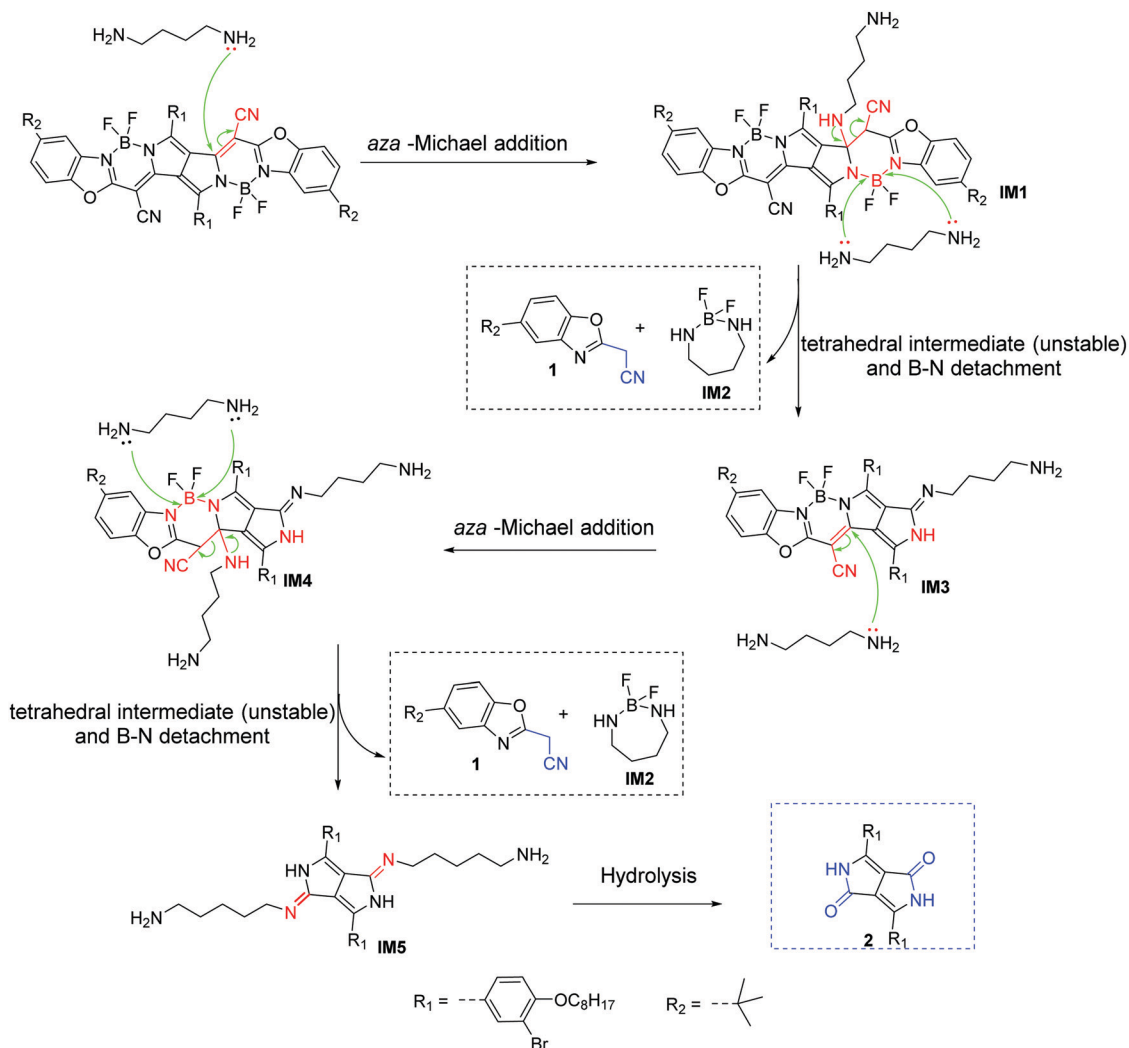
Scheme 2 The possible reaction mechanism between PPCy-1 and cadaverine.
