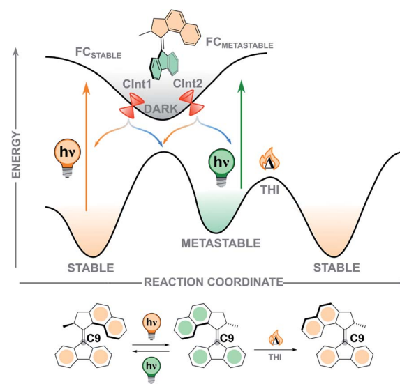
Fig. 7 Simplified potential energy surface (PES) along the isomerisation coordinate, showing the excited state processes occurring during the photochemical E - Z isomerisation. 117 The region of the perpendicular minimum is marked as "dark".
