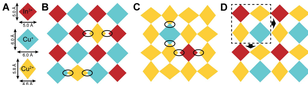
Fig. 4 Schematic top-down view of n = 1 perovskite sheets where [In III Cl 6 ] 3- , [Cu I Cl 6 ] 5- , and [Cu II Cl 6 ] 4- units are represented by red, blue, and yellow diamonds, respectively, with dimensions proportional to the coordination spheres found in the 300 K SCXRD structures of (PEA) 4 CuInCl 8 and (PCA) 2 CuCl 4 (A). (B) Packing arrangements for Cu 2+ doped into the Cu I –In III perovskite lattice and (C) Cu + and In 3+ doped into the Cu II perovskite lattice. Large packing mismatches are circled. (D) Proposed packing arrangement for 1 : One [In III Cl 6 ] 3- , one [Cu I Cl 6 ] 5- , and two [Cu II Cl 6 ] 4- units can be arranged into a cell and tessellated to yield a 2D lattice without large packing mismatch. See Fig. S9† for alternative tessellations of the same cell, which may explain the B-site disordering of 1 .
