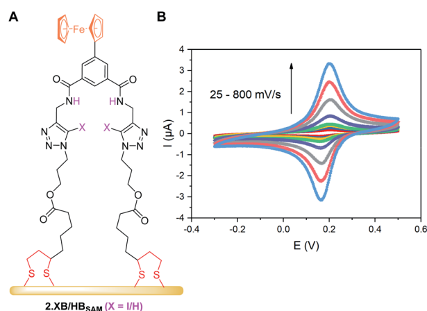
Fig. 4 (A) Schematic representation of 2.XB/HB SAM on a gold electrode. (B) CVs at varying scan rate of 2.HB SAM in ACN, 100 mM \text{TBAClO}_4 . The associated anodic and cathodic peak currents as a function of the square-root of the scan rate are shown in Fig. S25.†
