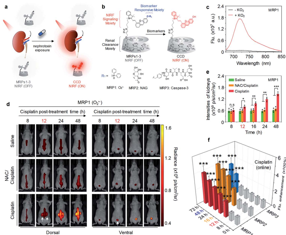
Fig. 5 (a) Schematic illustration of drug-induced AKI using MRPs1–3. (b) Chemical structures and molecular mechanisms of MRPs1–3 and their activated forms in response to O 2 •- , NAG and caspase-3, respectively, (R = H or CH 2 CHOHCH 3 ). (c) Fluorescence spectra of MRP1 (30 μM) in the absence or presence of KO 2 (60 μM) in PBS buffer (10 mM, pH 7.4). (d) Representative NIR fluorescence images of living mice with injection of MRP1 after treatment of cisplatin (20 mg per kg body weight) for 8, 12, 24 or 48 h. The control groups were treated with PBS or a nephroprotective antioxidant NAC. NIRF images acquired at 720 nm upon excitation at 675 nm. (e) NIRF intensities of kidneys in living mice after 30 min injection of MRP1 at the different post-treatment time points (8, 12, 16, 24 or 48 h). (f) Fluorescence enhancement of excreted MRPs1–3 in the urine from cisplatin-treated living mice after injection at different time points post-treatment of cisplatin. n.s.: not significant, * p < 0.05, ** p < 0.01, *** p < 0.001. Reproduced with permission from ref. 56. Copyright 2019 Springer Nature.
