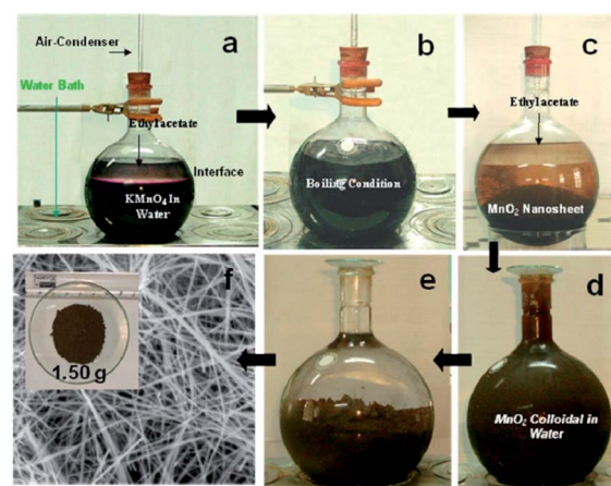
Fig. 2 Preparation of gram level \alpha -MnO 2 nanowires from aqueous KMnO 4 /ethyl acetate biphasic system and their different stages (a–f) in digital/FESEM images. Reproduced by Sinha et al. 65 with permission from ACS.
