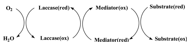
Fig. 3 Typical catalytic mechanism of LMS.
